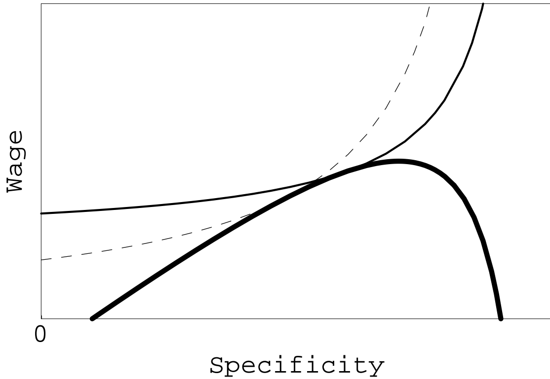
Figure 2: An increase in unemployment income flattens workers' indifference curves, from the dashed line to the solid line, shifting the tangency point towards higher wages and specificity.
