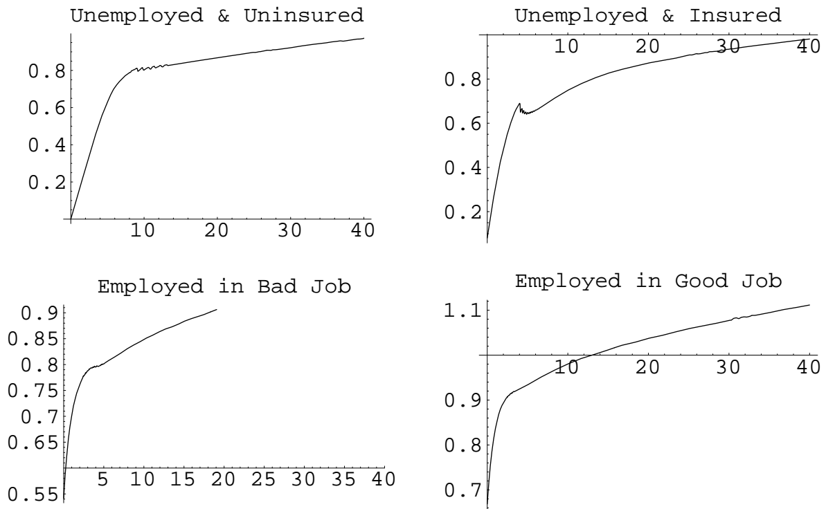
Figure 3: Consumption as a function of normalized assets in the four employment states, benchmark parameterization. Note that workers quit bad jobs when their assets exceed 19.
