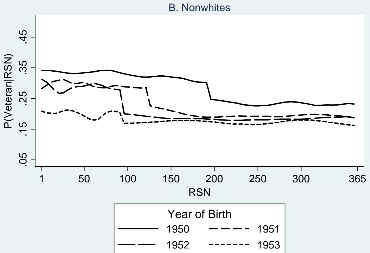
Figure 1. First-stage plots (bandwidth=.4). The relation between the probability of military service and draft lottery numbers. Data from the 2000 Census.
