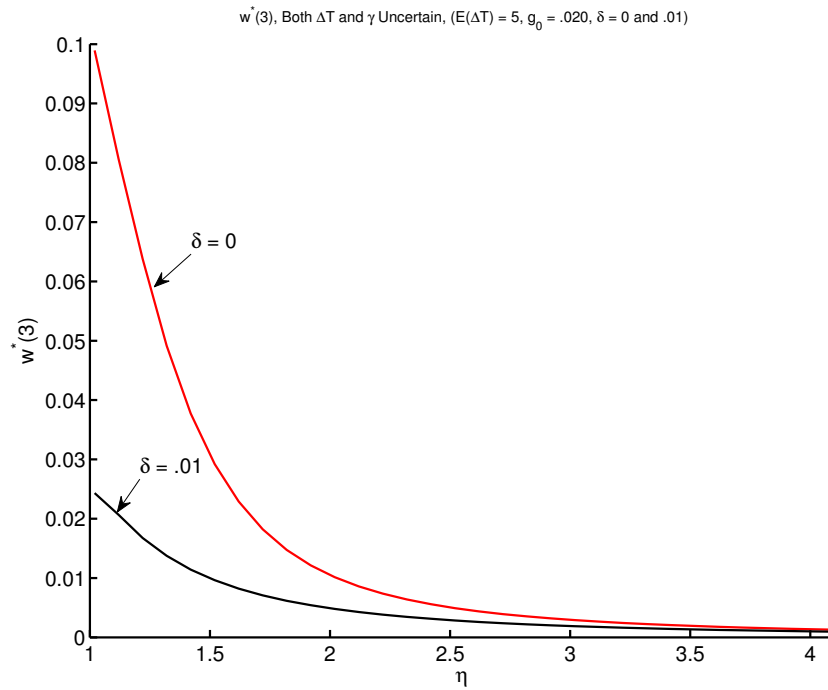
Figure 9: WTP Versus \eta for \tau = 3 . \mathcal{E}(\Delta T_H) = 5^\circ\text{C} , H = 100 , g_0 = .020 , \delta = 0 and .01
