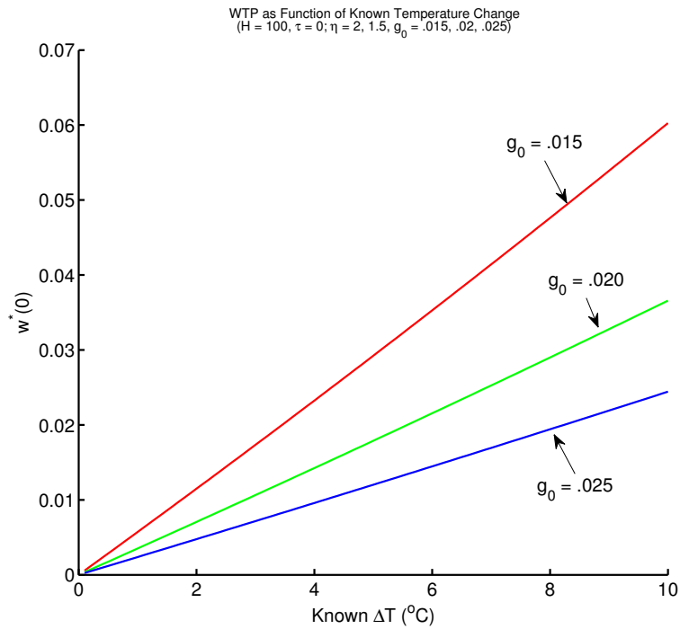
Figure 4: WTP, Known Temperature Change, \eta = 2 , g_0 = .015, .020, .025 , and \delta = 0
