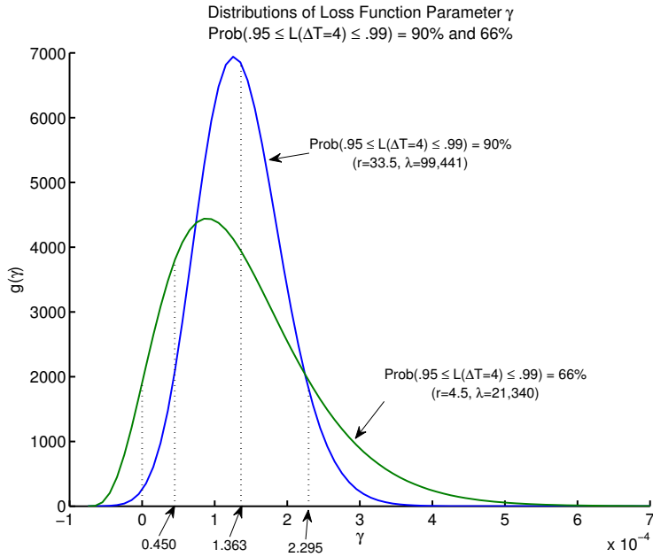
Figure 3: Distributions for Loss Function Parameter \gamma
