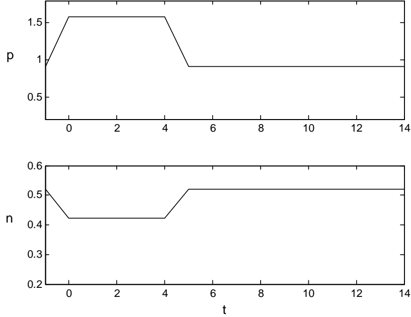
Figure 2: First Best
