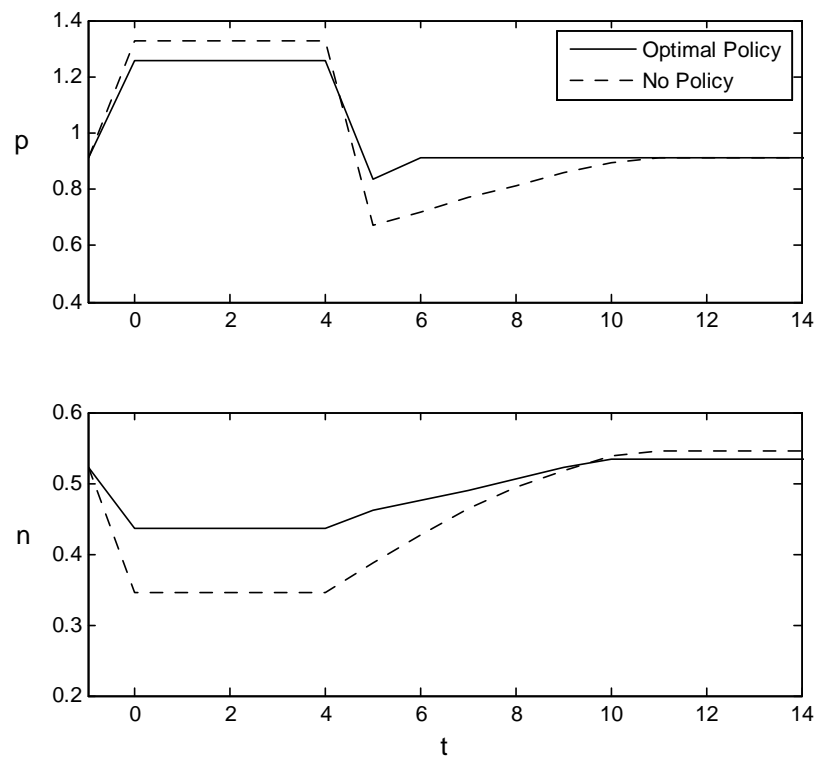
Figure 5: Optimal Policy
